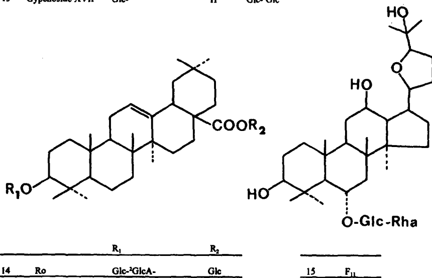
Fig. 1. Structures of ginsenosides referred to in Section 1.
